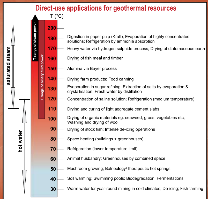
Figure 1: Examples of direct-use applications for geothermal energy (modified from Lindal (1973)) [1] .
