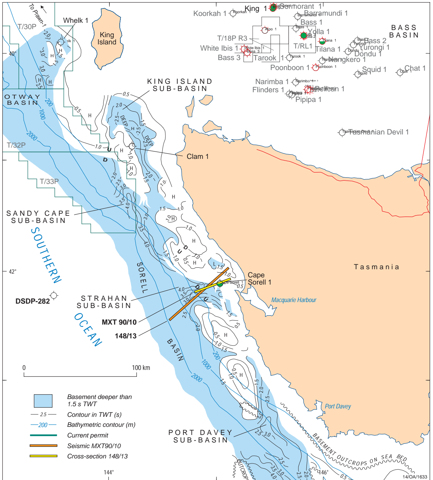
Sediment thickness and cross-section locations, Sorell Basin (modified after Lodwick et al, 1999).
