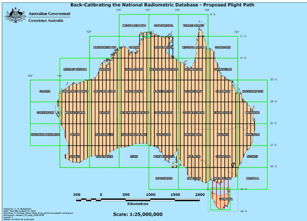
Figure 1. Proposed flight line pattern for the AWAGS 2 magnetics and radiometrics survey to back-calibrate the National Radiometric Database
